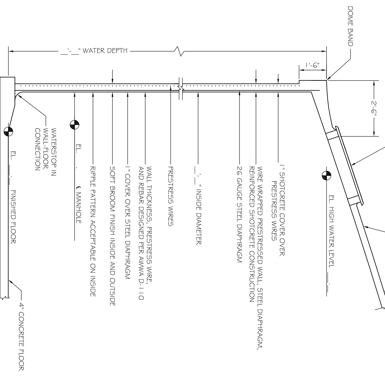
TANK SECTION NTS
